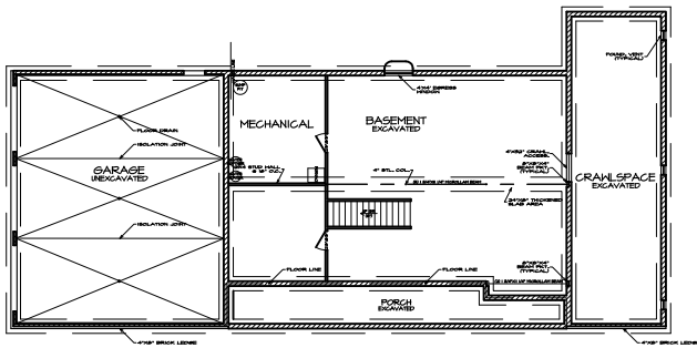
FOUNDATION PLAN
